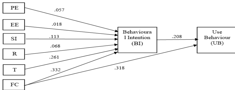
Figure 2: Structural Model (UTAUT + Risk Perception + Trust) with Standardized Coefficients
