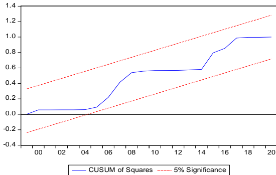
Figure 3. Result of CUSUM test of square (Author's work based on EViews package)
