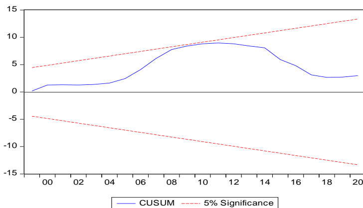
Figure 2. Result of CUSUM test (Author's work based on EViews package)
