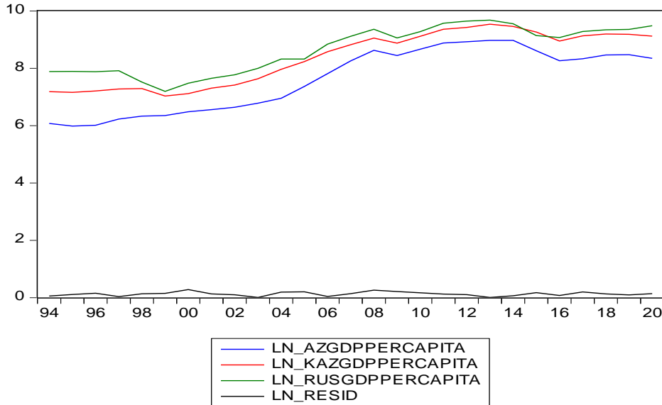
Figure 1. Dynamic graph of indicators (Author's work based on EViews package)
